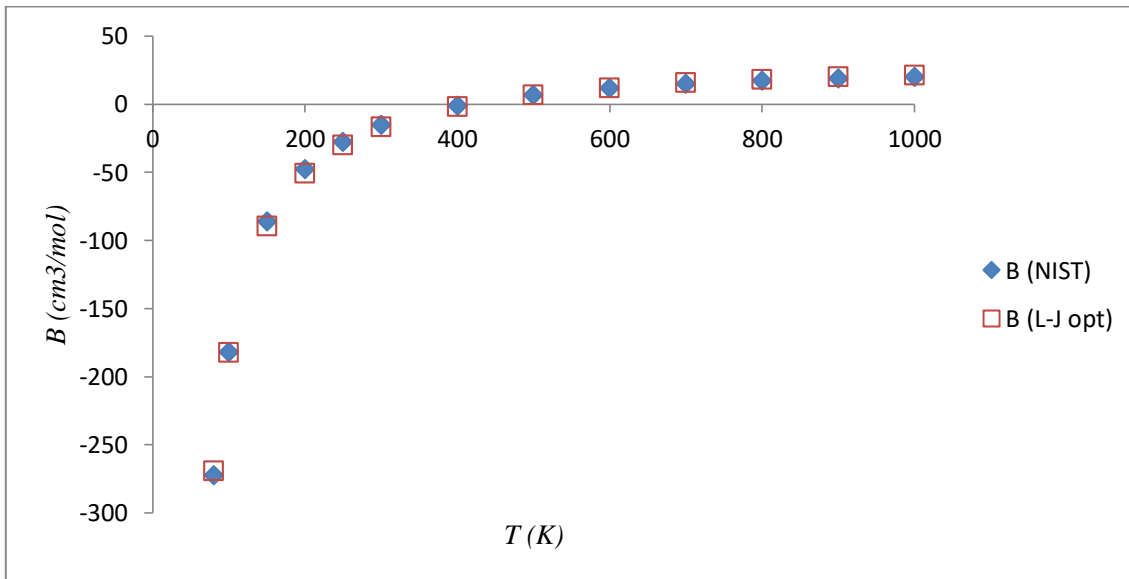
Figure 12. Graphical comparison of B(T) values for argon, against L-J potential.
