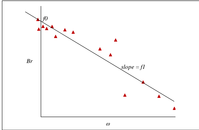
Figure 2. Expected relationship between B_r and \omega for a normal fluid.
