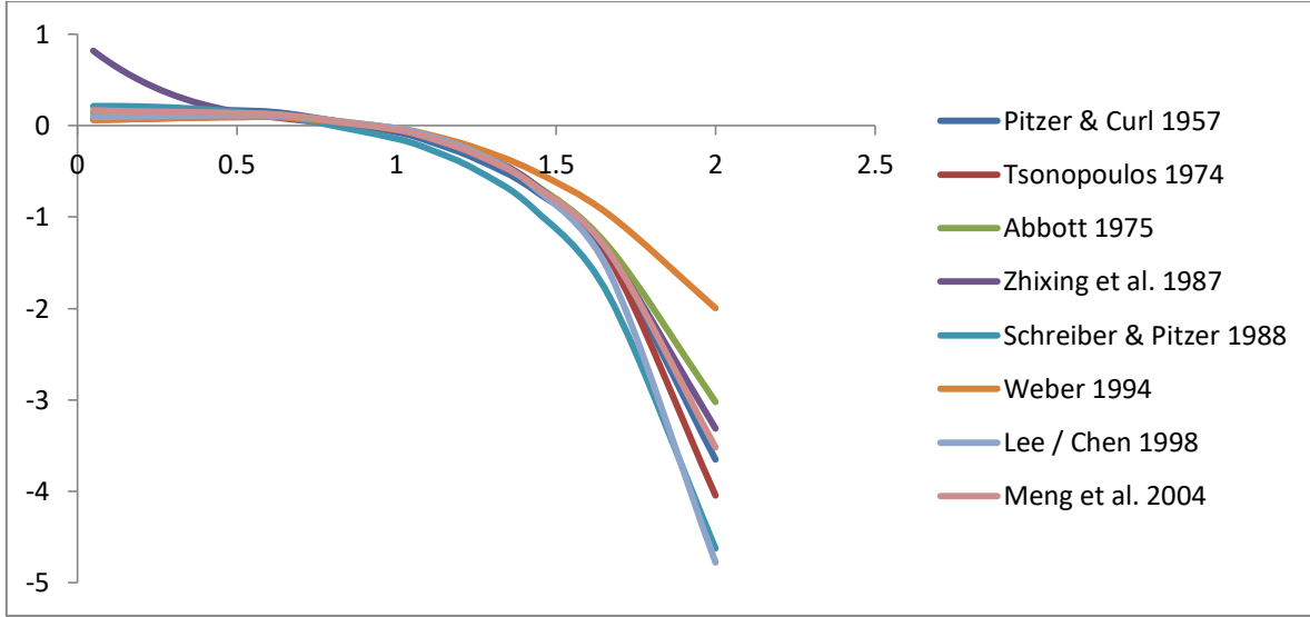
Figure 17. Graphical comparison of different f_1 functions.
