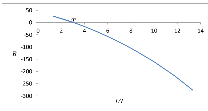
Figure 4. Typical graph of B vs 1/T for nitrogen.
