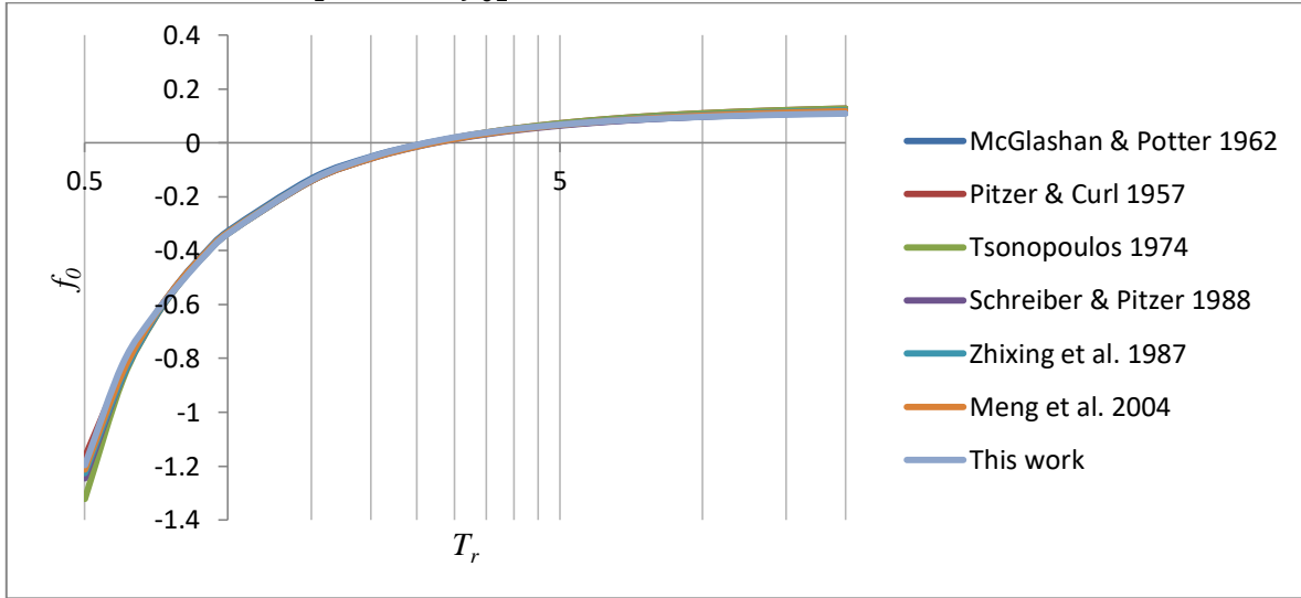
Figure 59. Comparison of f_{01} from this work with other correlations.
