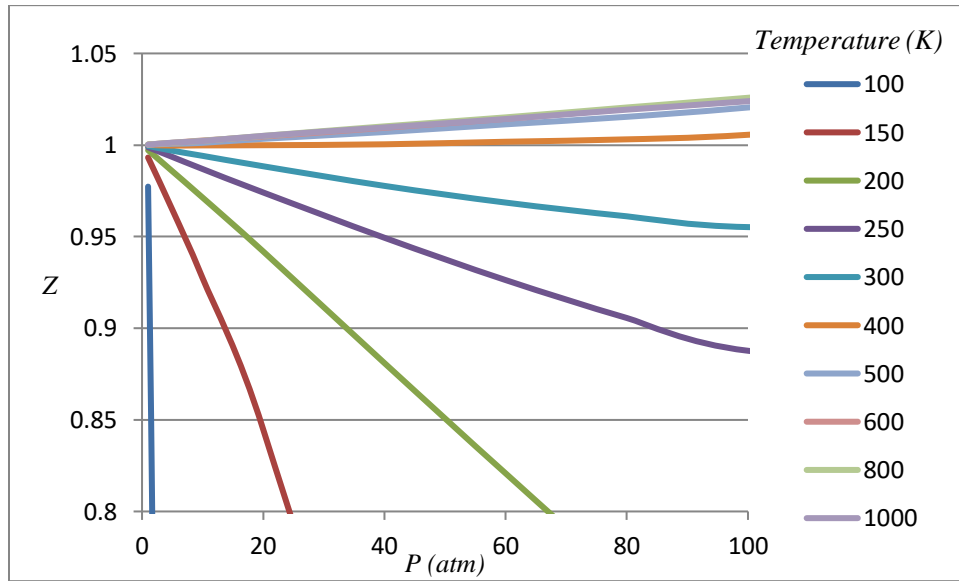
Figure 1. Variation of argon compressibility with pressure, at several temperatures. Data from Perry & Green (2007).
