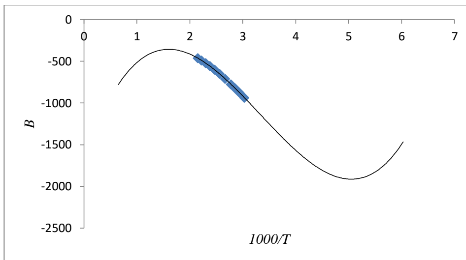
Figure 24. Uranium hexafluoride, data and fit by Dymond et al. (2002).
