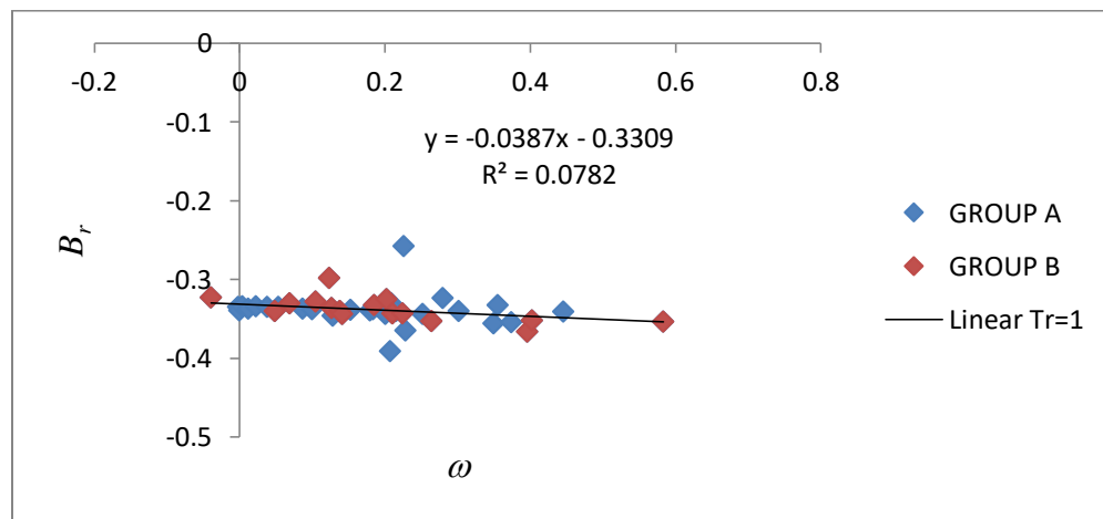
Figure 65. B_{r2} versus acentric factor at T_r = 1 .
