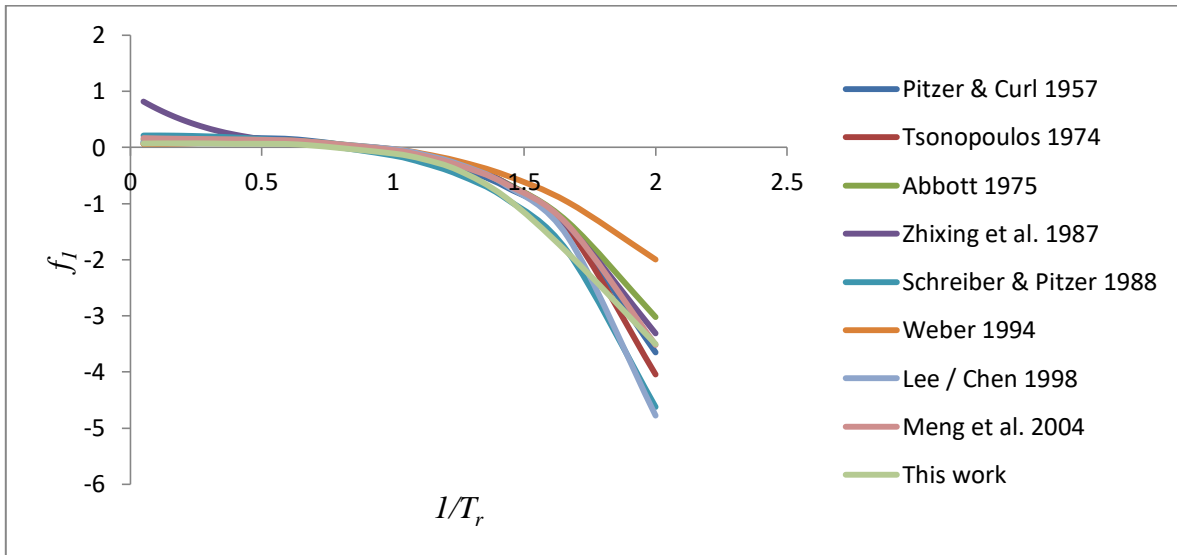
Figure 61. Comparison of f_1 from this work with other correlations.
