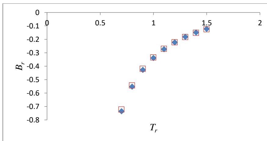
Figure 77. Comparison of B_{r2} values for propene.
