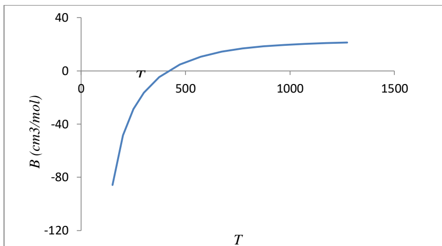
Figure 3. Typical graph of B vs. T for argon.
