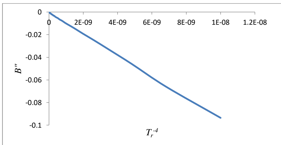
Figure 25. Second derivative of B for argon (data from NIST).
