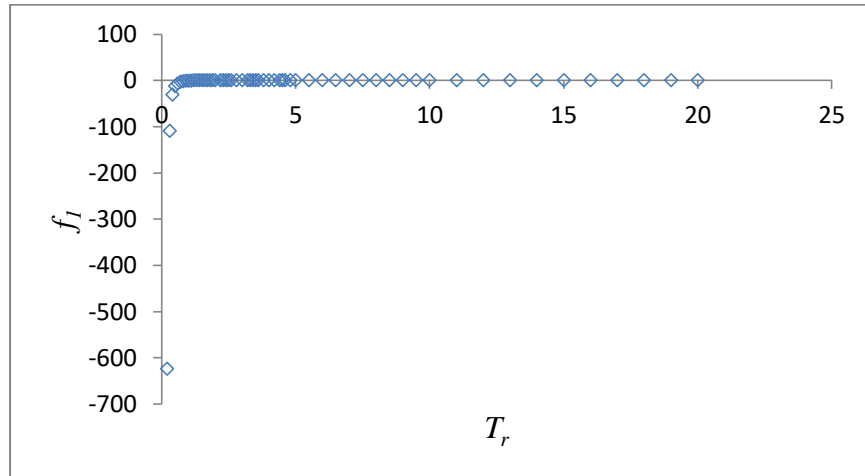
Figure 44. Function f_{11} versus T_r for correlation in V_c .
