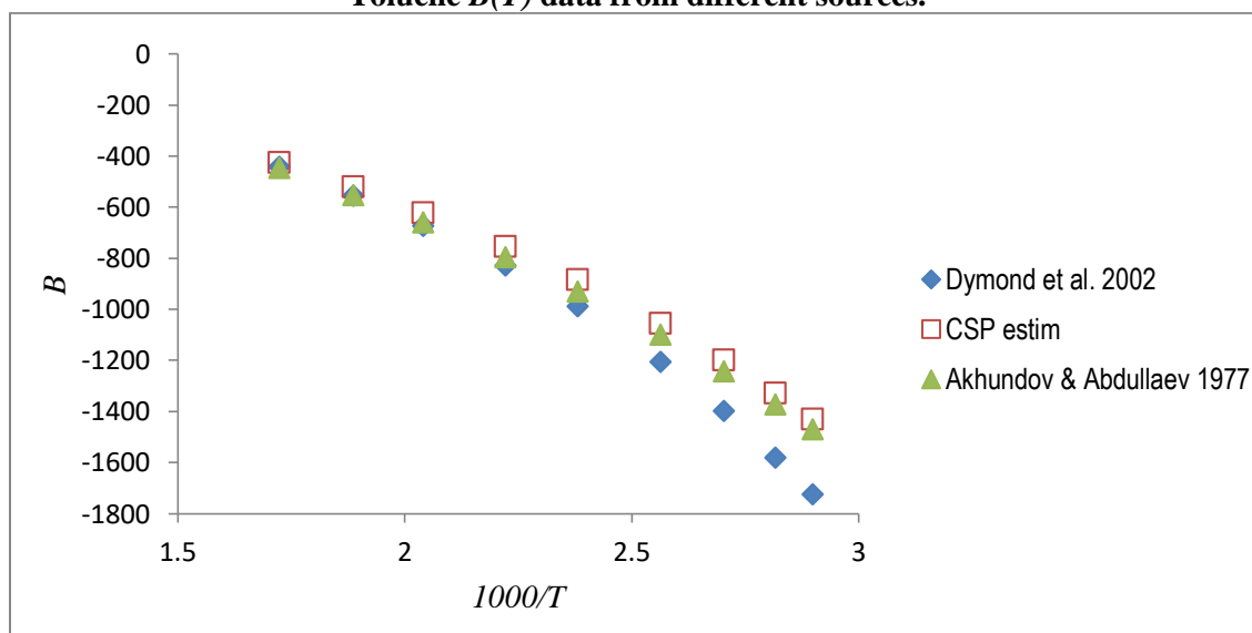
Figure 36. Toluene B(T) data from different sources.
