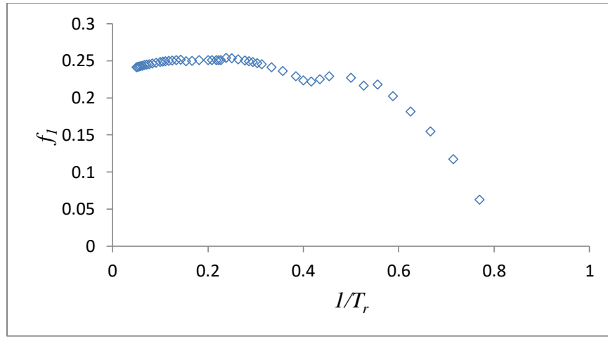
Figure 48. Close-up of Figure 44.
