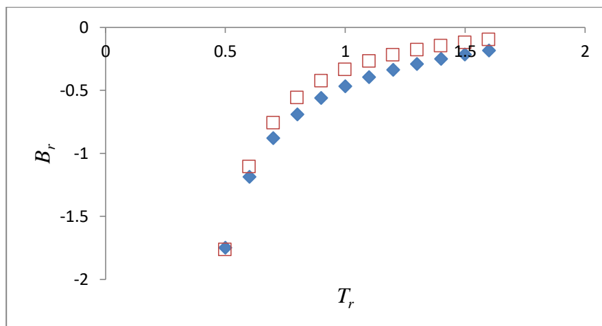
Figure 80. Comparison of B_{r2} values for tetrachloromethane.
