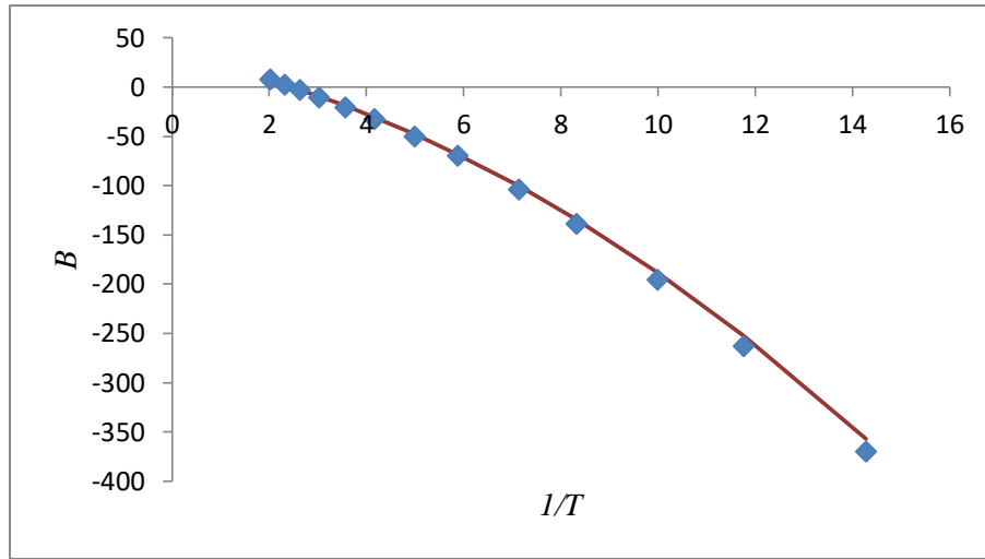
Figure 14. Comparison of Eq. (38A) against oxygen B(T) data (Dymond et al. 2002).
