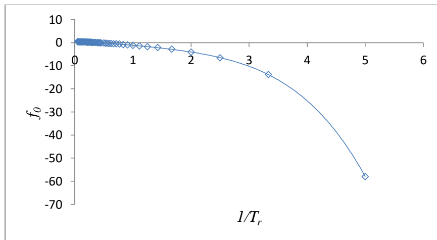
Figure 45. Function f_{01} versus 1/T_r for correlation in V_c .
