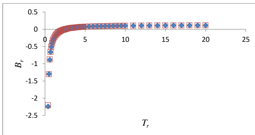
Figure 76. Comparison of B_{r2} values for nitrogen.
