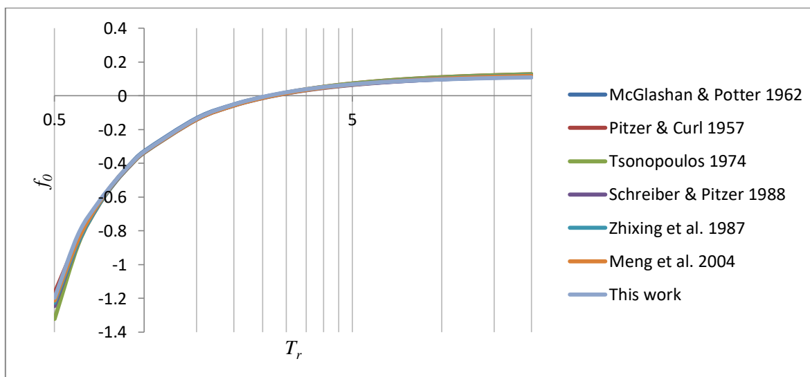
Figure 84. Comparison of f_{02} from this work with other correlations.
