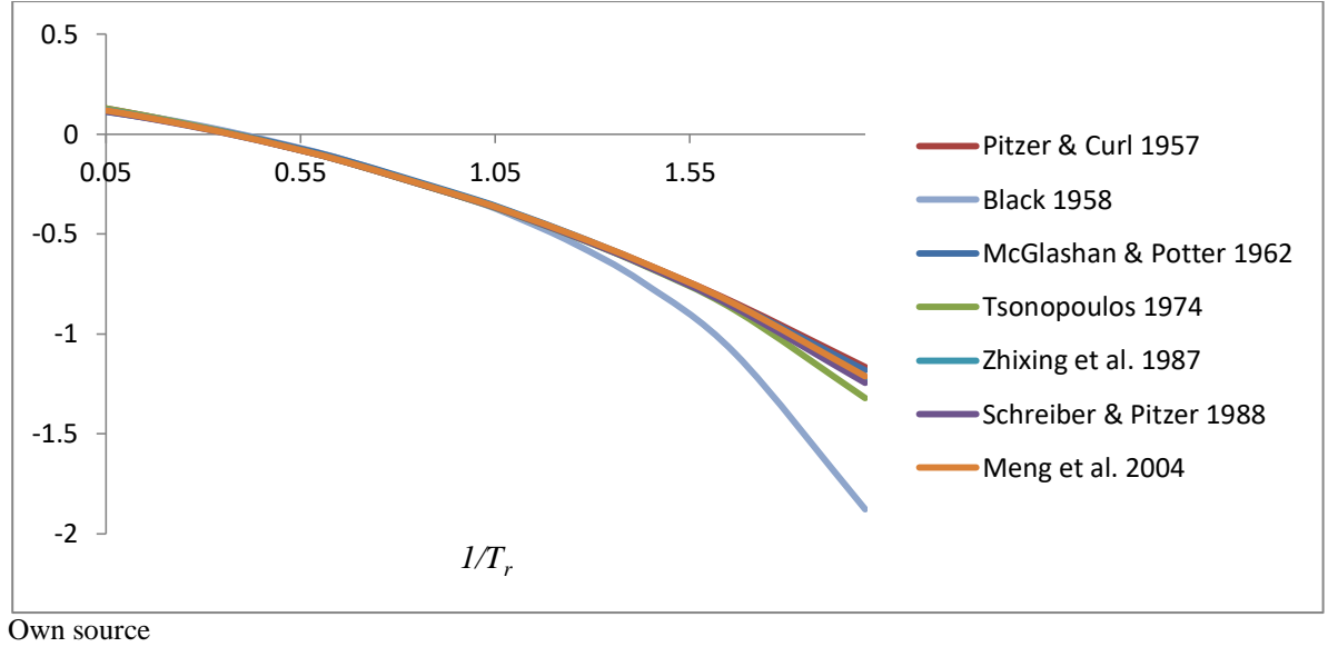
Figure 16. Graphical comparison of different f_0 functions.
