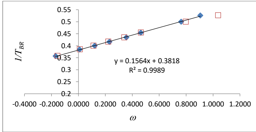
Figure 75. Reduced Boyle temperature versus \omega .
