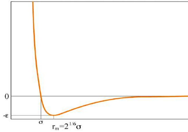
Figure 9. Lennard-Jones potential.
