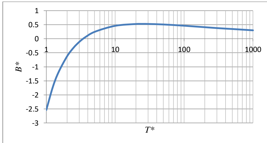
Figure 10. Lennard-Jones reduced second virial coefficient.
