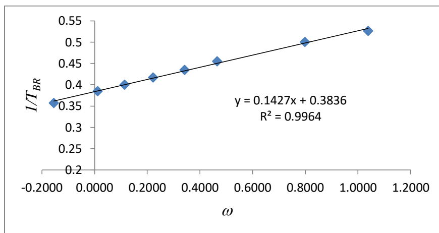
Figure 50. Reduced Boyle temperature versus \omega .
