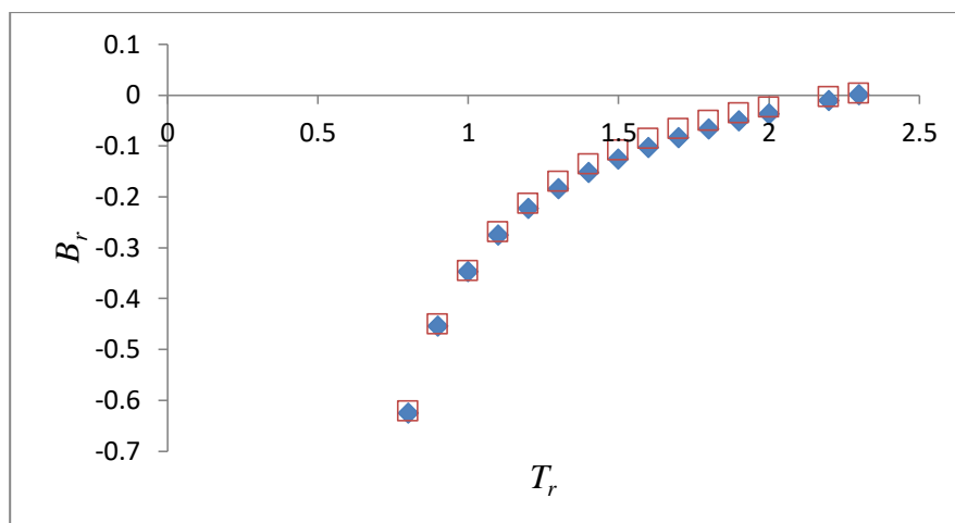
Figure 79. Comparison of B_{r2} values for octane.
