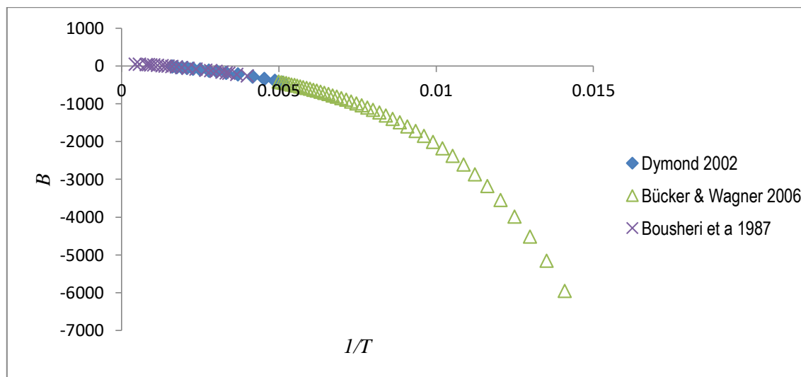
Figure 30. Available B(T) data for ethane.
