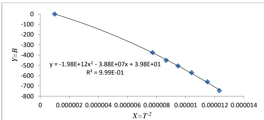
Figure 35. Temperature dependence of B(T) for 1,3-butadiene.
