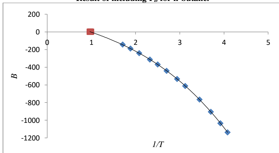
Figure 32. Result of including T_B for n-butane.
