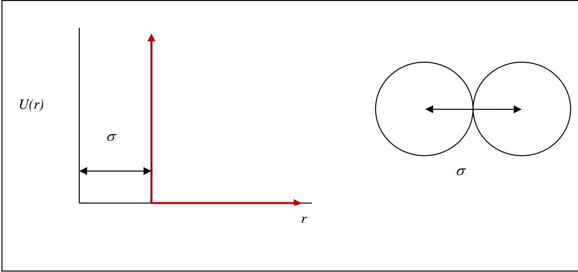
Figure 7. Hard-spheres potential.
