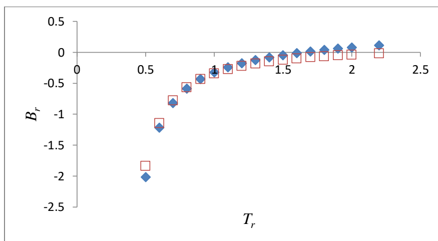
Figure 82. Comparison of B_{r2} values for trans-2-butene.
