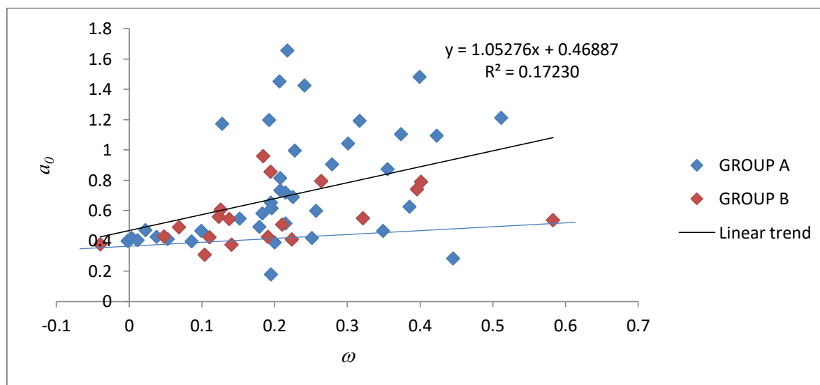
Figure 37. Plot of a_0 reduced on V_c versus \omega , all substances.
