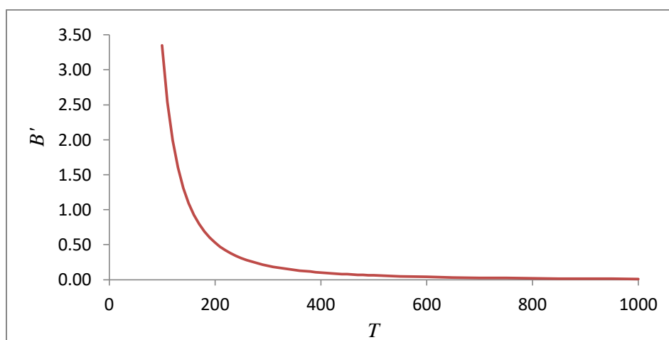
Figure 5. The first derivative of B(T) for argon.
