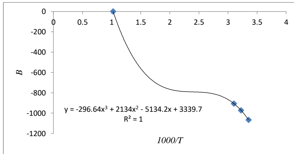
Figure 19. Oscillatory behavior and inflexion point.
