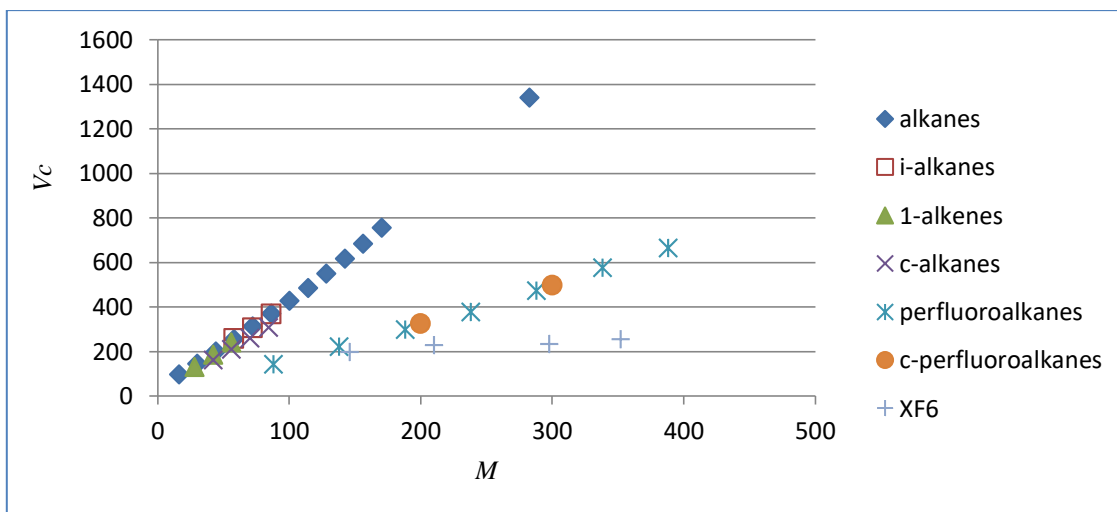
Figure 11. Validation of the critical volume data.
