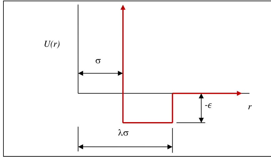
Figure 8. Square well potential.
