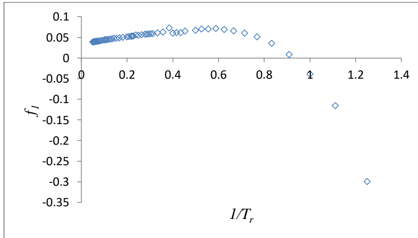
Figure 73. Close-up of Figure 69.
