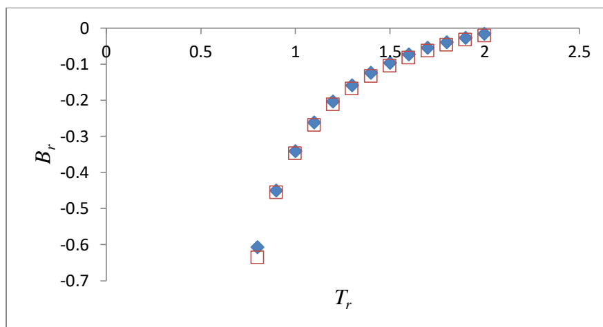
Figure 83. Comparison of B_{r2} values for cycloperfluorohexane.
