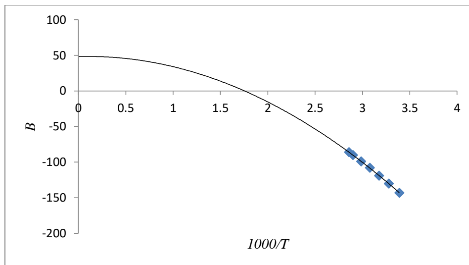
Figure 22. Silicon tetrafluoride, data and fit by Dymond et al. (2002).
