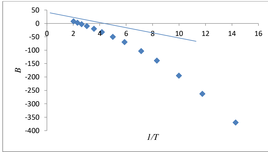
Figure 18. Expected behavior of B(T) , oxygen data (Dymond et al. 2002).
