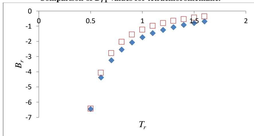
Figure 55. Comparison of B_{r1} values for tetrachloromethane.
