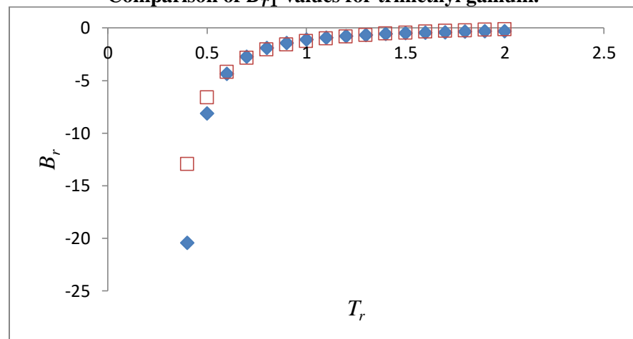
Figure 56. Comparison of B_{r1} values for trimethyl gallium.
