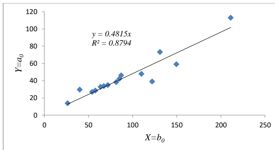
Figure 31. Comparison between optimum values of a_0 vs. Lennard-Jones b_0 .
