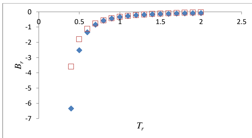
Figure 81. Comparison of B_{r2} values for trimethyl gallium.
