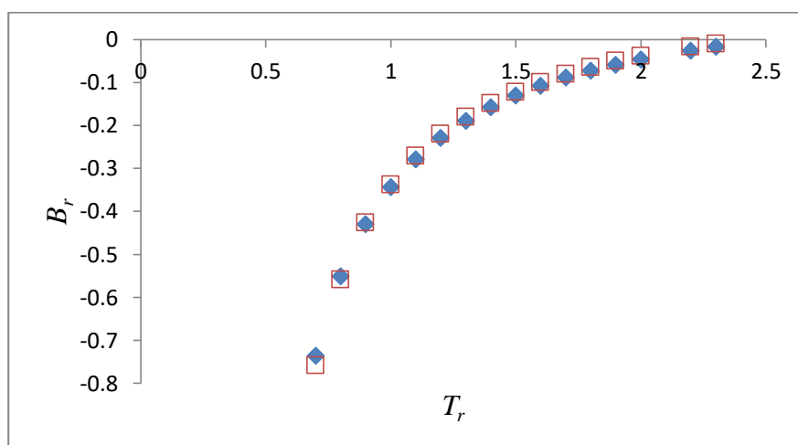
Figure 78. Comparison of B_{r2} values for acetylene (ethyne).
