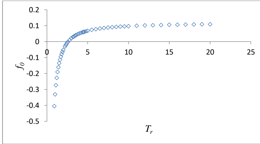
Figure 72. Close-up of Figure 66.
