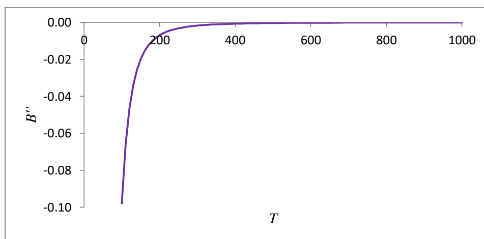
Figure 6. The second derivative of B(T) for argon.
